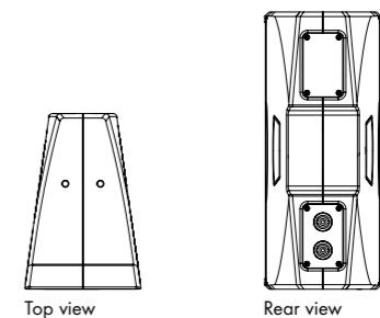
Ti10P cabinet dimensions in mm [inch]
