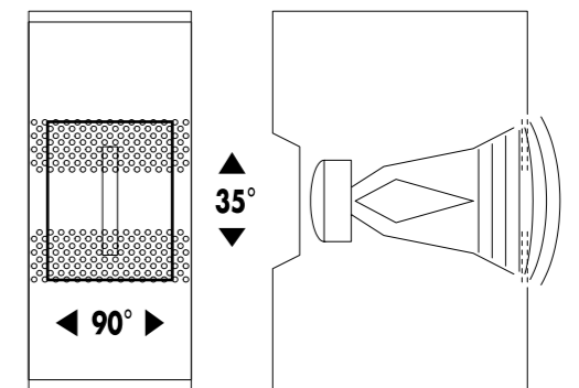
T10 horn and lens in point source setup
