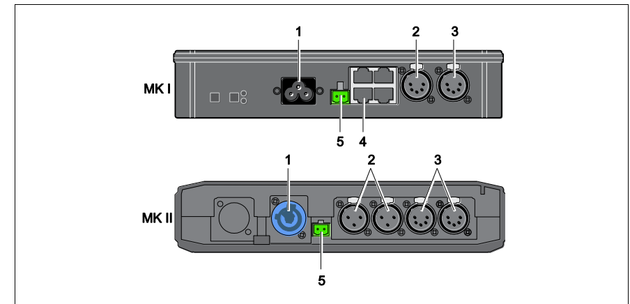
Fig. 7: Connectors and ports of BlackBox R-512
