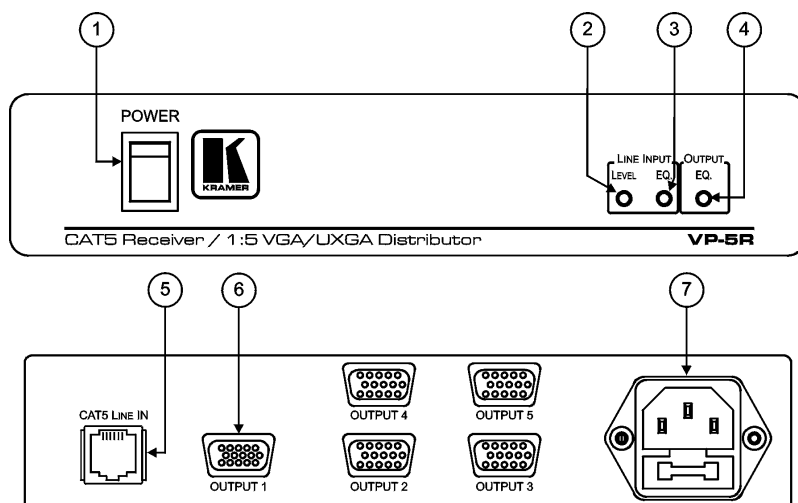
Figure 5: VP-5R CAT 5 Receiver/1:5 VGA/UXGA Distributor
