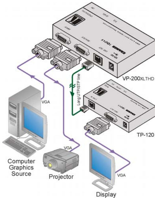
Figure 7: Connecting the VP-200XLTHD
