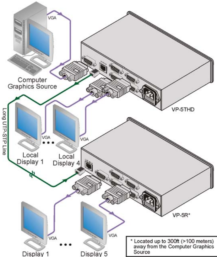
Figure 8: Connecting the VP-5THD and the VP-5R
