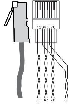
Figure 9: TP Connector
